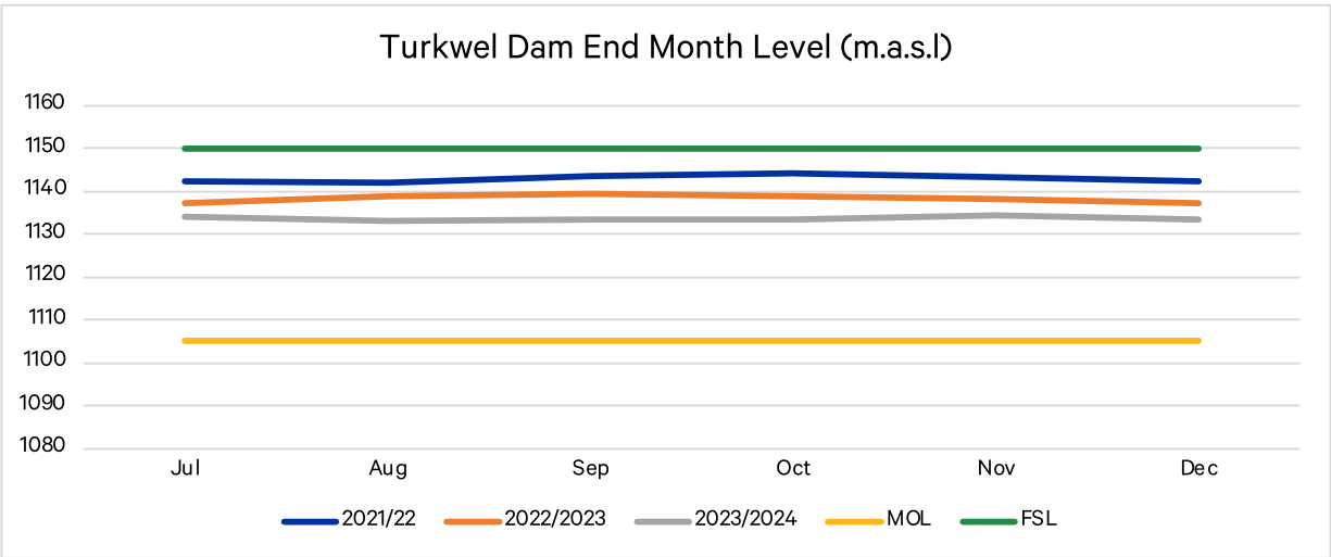
Figure 2.5: Turkwel dam levels between July and December 2023
