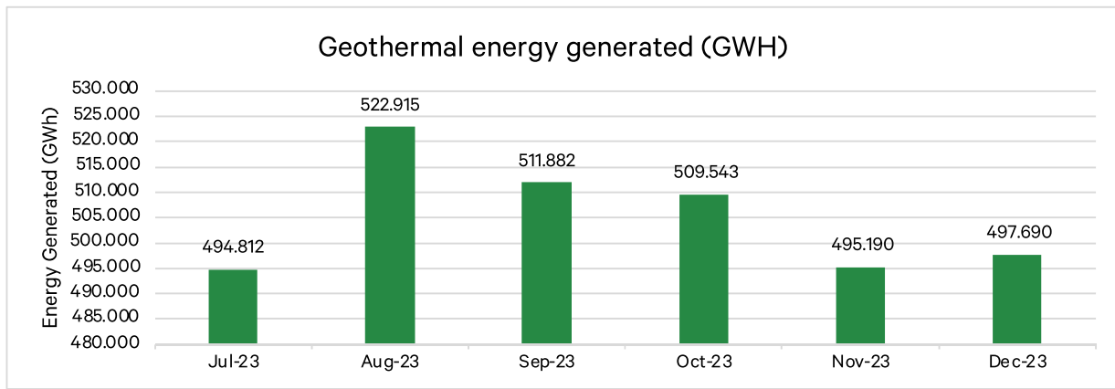
Figure 2.2: Geothermal energy generated between July and December 2023
