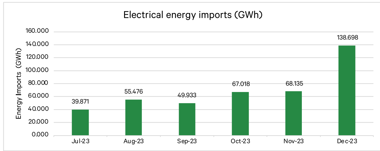
Figure 4.1: Electrical energy imports between July and December 2023
