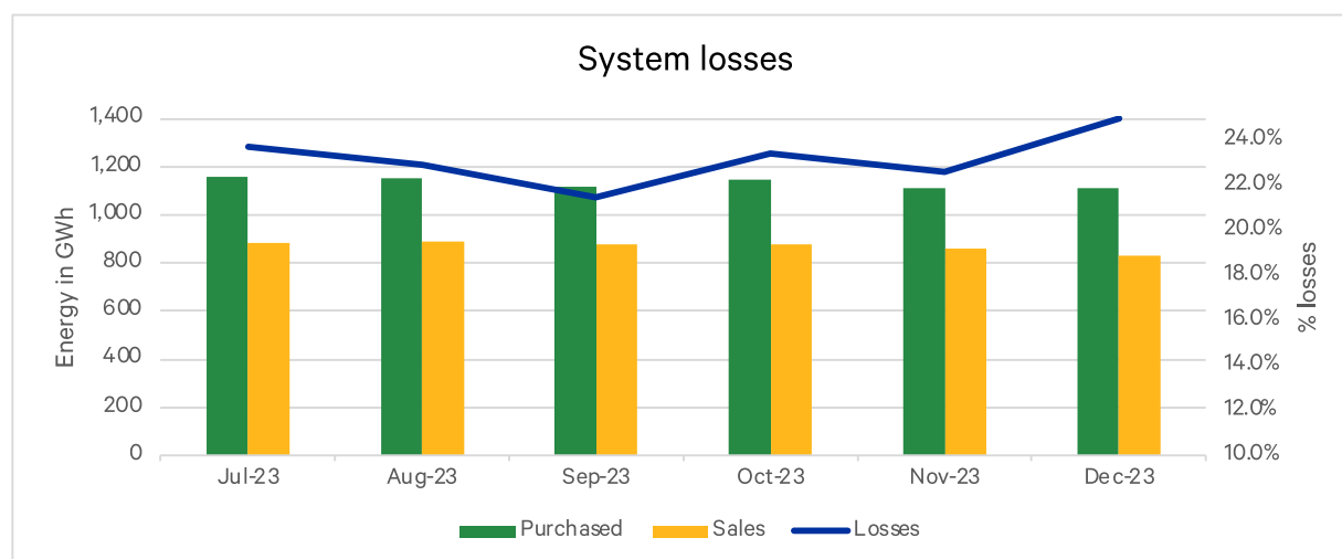
Figure 1.9: System losses between July and December 2023
