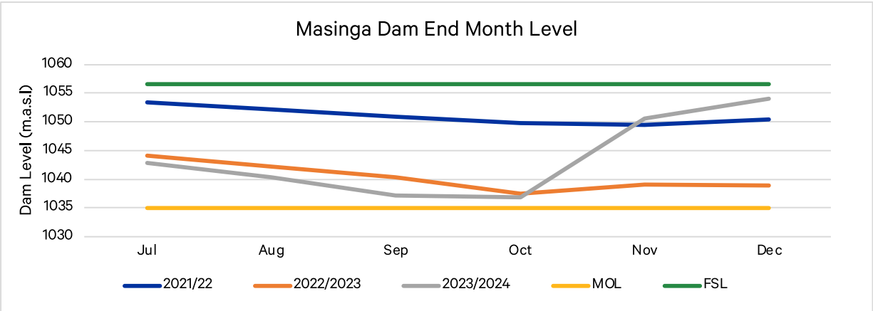
Figure 2.6: Masinga dam levels between July 2021 and December 2023
