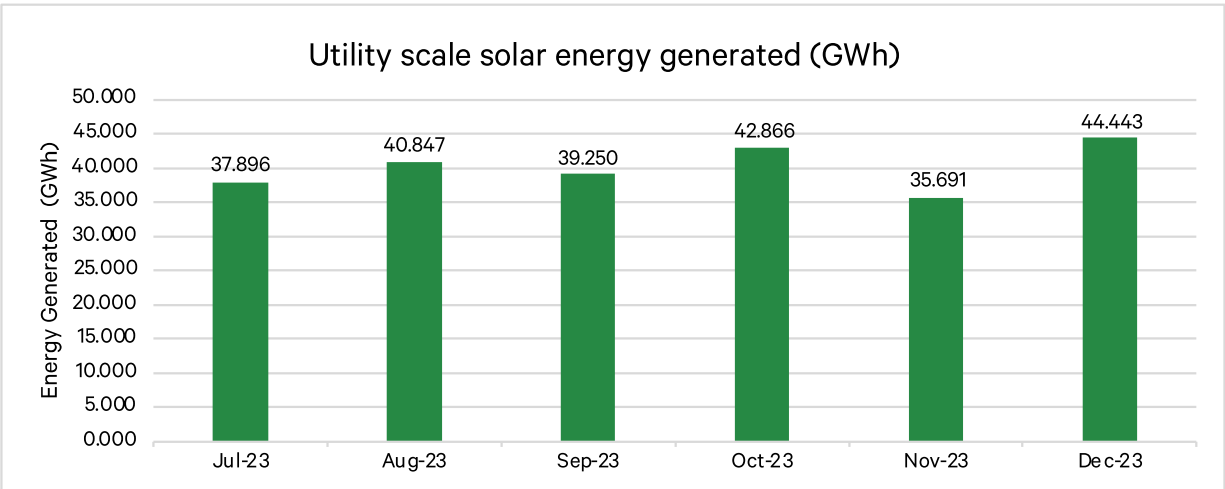
Figure 2.10: Solar energy generation between July and December 2023
